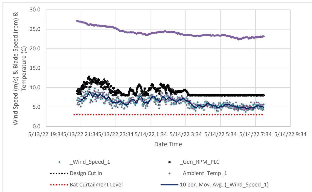
WTG0004 Time Series Plot of Ambient Temperature, Wind Speed, and Blade Roter Speed
