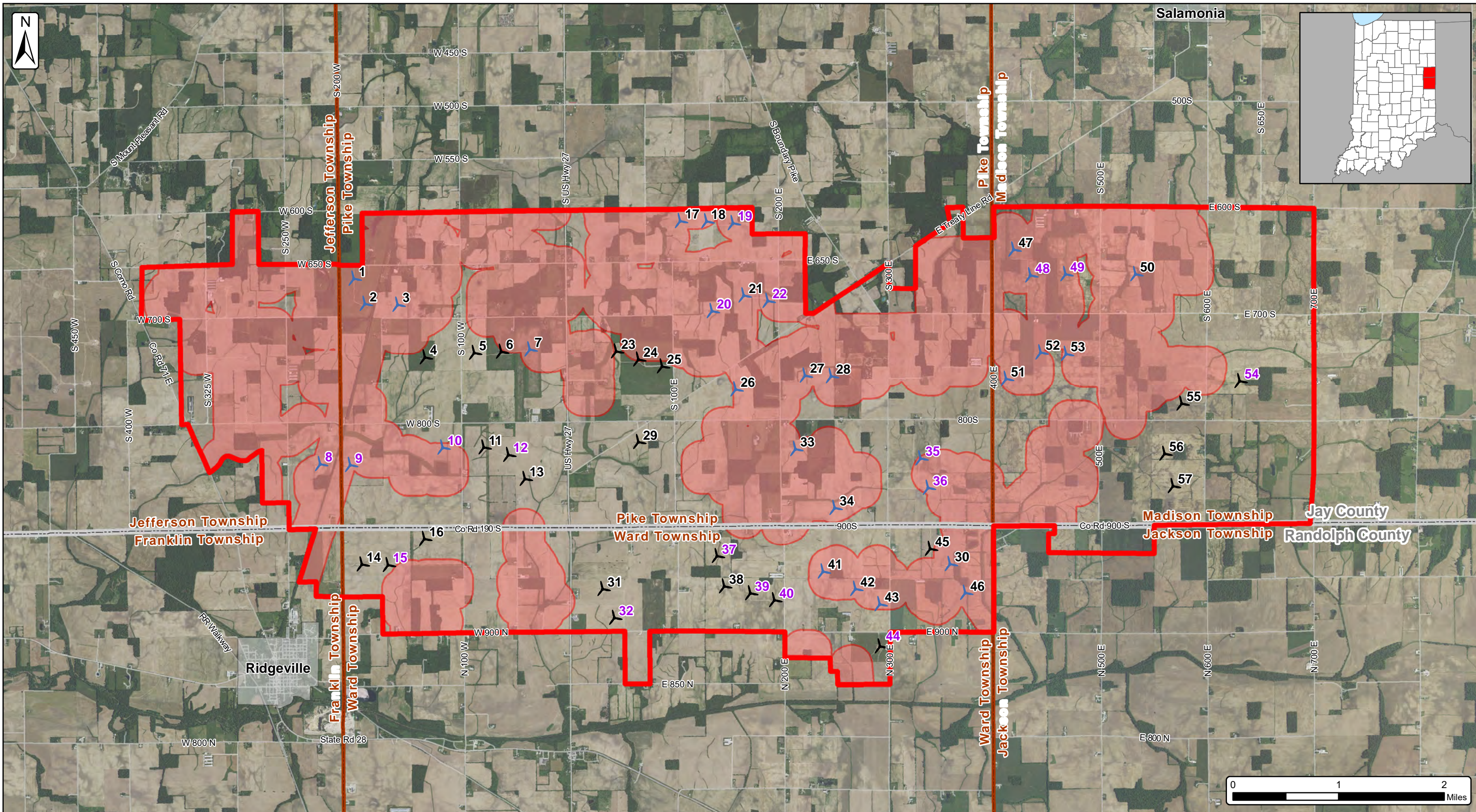
Bluff Point Wind Energy Center Figure 3 As-Built Turbines and Bat Fatality Search Locations Jay & Randolph Counties, Indiana Date: 12/8/2022
