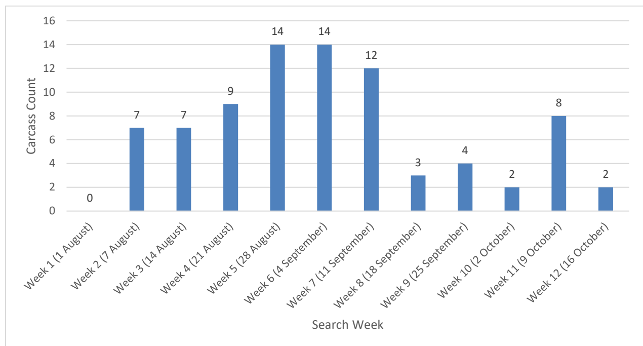
Figure 2. Bat carcasses found by week during the 2023 post-construction standardized surveys (1 Aug through 17 October) at the Wildcat Wind Farm, Tipton and Madison counties, Indiana.
