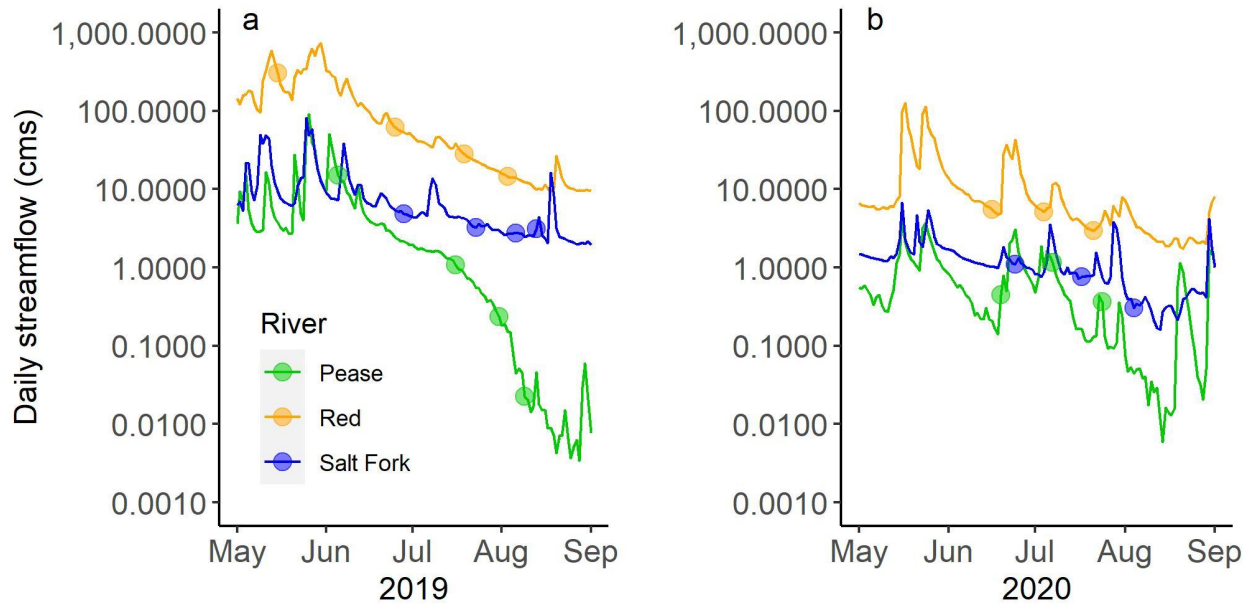
Figure 7. Hydrographs for the Red River (U.S. Geological Survey gage # 07308500), Salt Fork Red River (USGS gage # 07301110), and Pease River (USGS gage # 07308200) indicating daily discharge from May through September of (a) 2019 and (b) 2020 (U.S. Geological Survey, 2020). Lines are colored by river and similarly colored points on lines represent sampling dates. Note the y-axis is shown on a \log_{10} scale.
