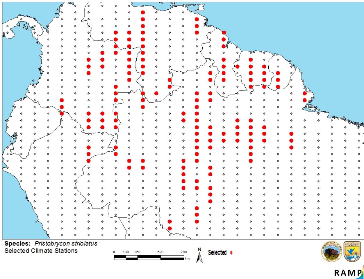
Figure 2. RAMP (Sanders et al. 2018) source map showing weather stations in South America selected as source locations (red; Colombia, Venezuela, French Guiana, Guyana, Suriname, Brazil, Peru) and non-source locations (gray) for Pristobrycon striolatus climate matching. Source locations from GBIF Secretariat (2018). Selected source locations are within 100 km of one or more species occurrences, and do not necessarily represent the locations of occurrences themselves.
