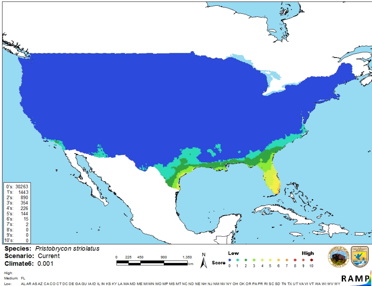
Figure 3. Map of RAMP (Sanders et al. 2018) climate matches for Pristobrycon striolatus in the contiguous United States based on source locations reported by GBIF Secretariat (2018). Counts of climate match scores are tabulated on the left. 0/Blue = Lowest match, 10/Red = Highest match.
