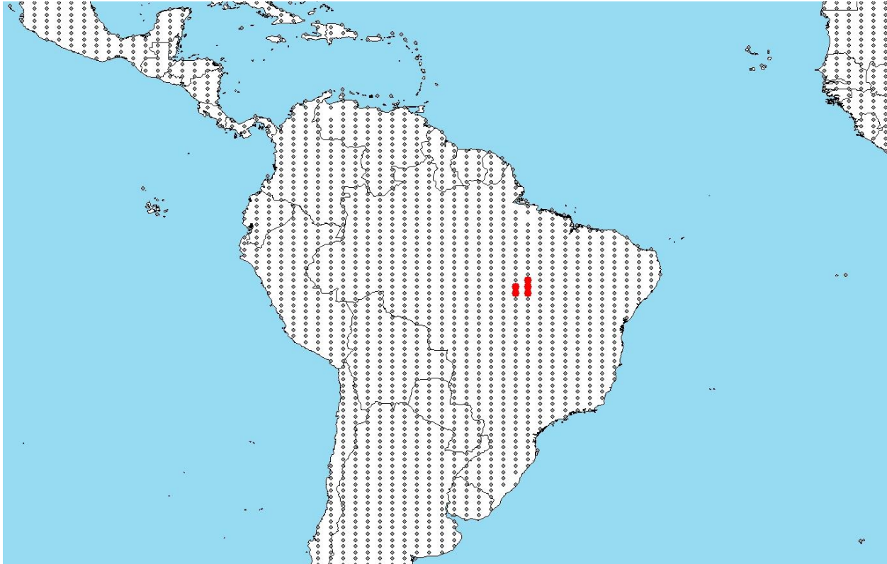
Figure 2. RAMP (Sanders et al. 2018) source map showing weather stations in South America selected as source locations (red; Brazil) and non-source locations (gray) for S. geryi climate matching. Source locations from GBIF Secretariat (2017).
