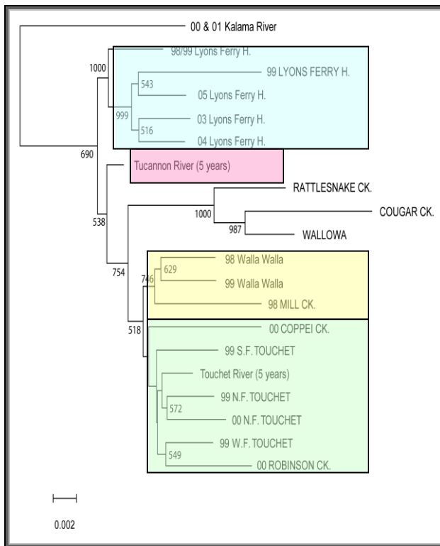
Figure 2. Chord distance tree from steelhead samples from Columbia River, Walla Walla River, and Snake River. Sample labels with all letters capitalized are juvenile samples. Node support numbers are values from bootstrap analysis (1000 bootstraps).
