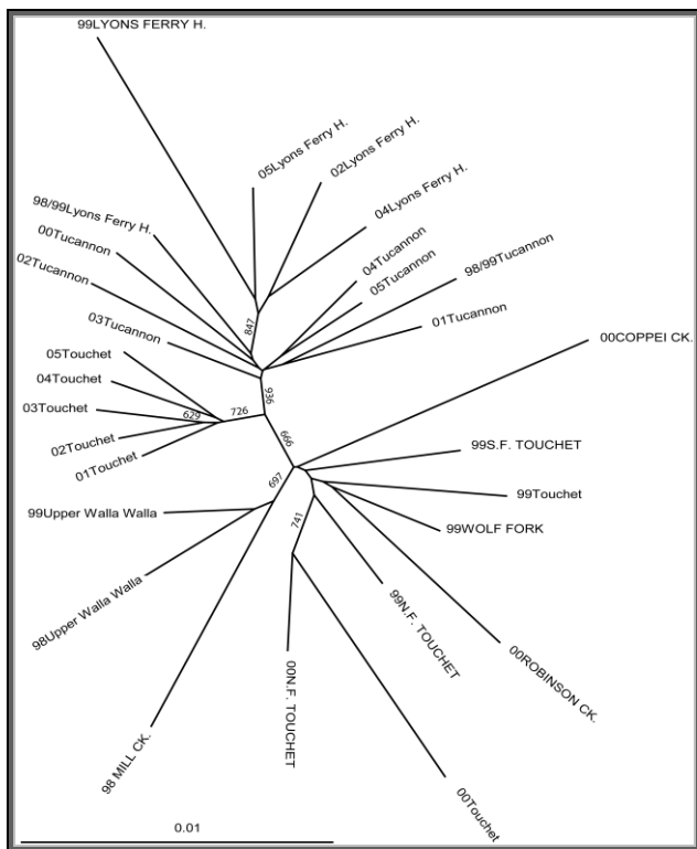
Figure 1. Chord distance tree that includes temporally stratified samples (from Figure 2), plus samples from Touchet River tributaries, Mill Creek, and Walla Walla River. Sample labels with all letters capitalized are juvenile samples. Node support numbers are values from bootstrap analysis (1000 bootstraps).
